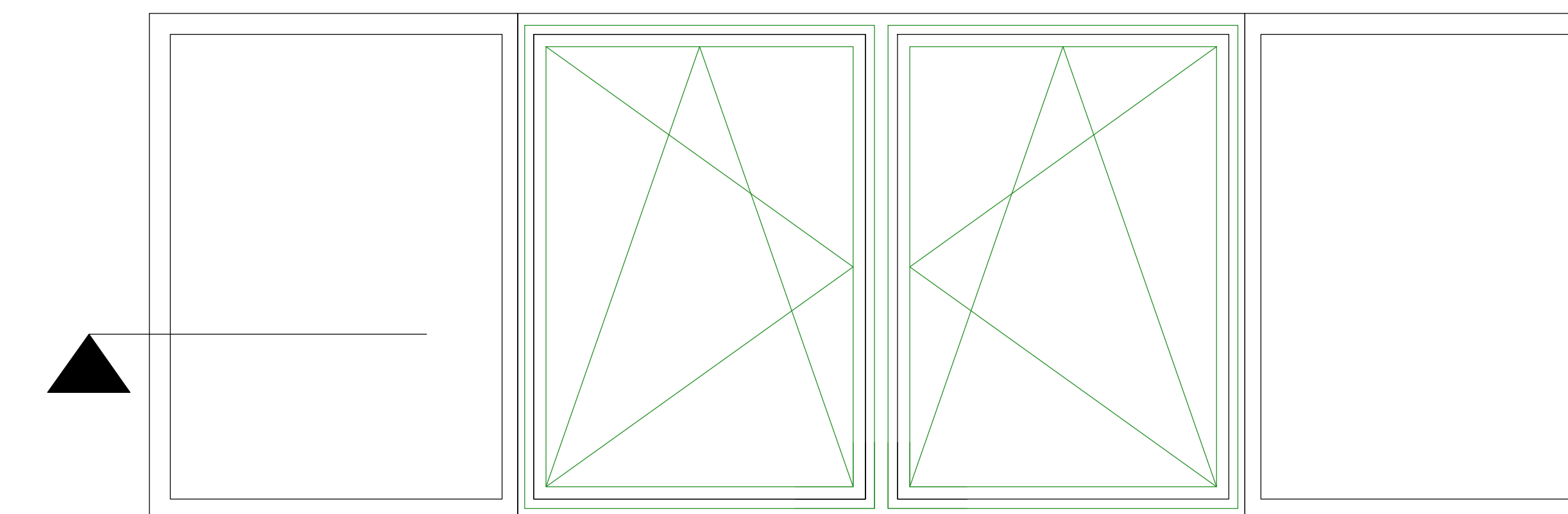
EXPANSION MULLION
