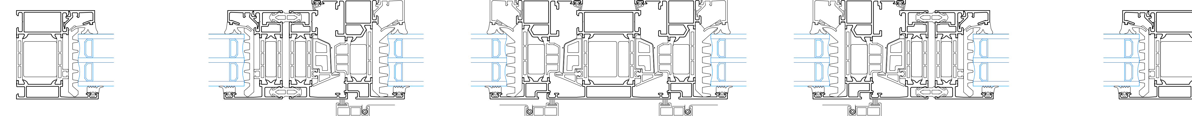
EXPANSION MULLION
